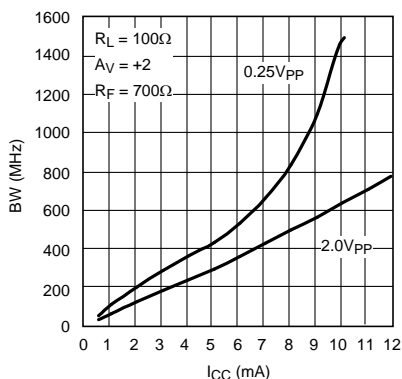
Figure 1. -3dB BW vs. I_{CC}
